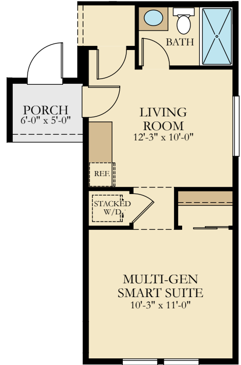
OPT. MULTI-GEN SUITE
