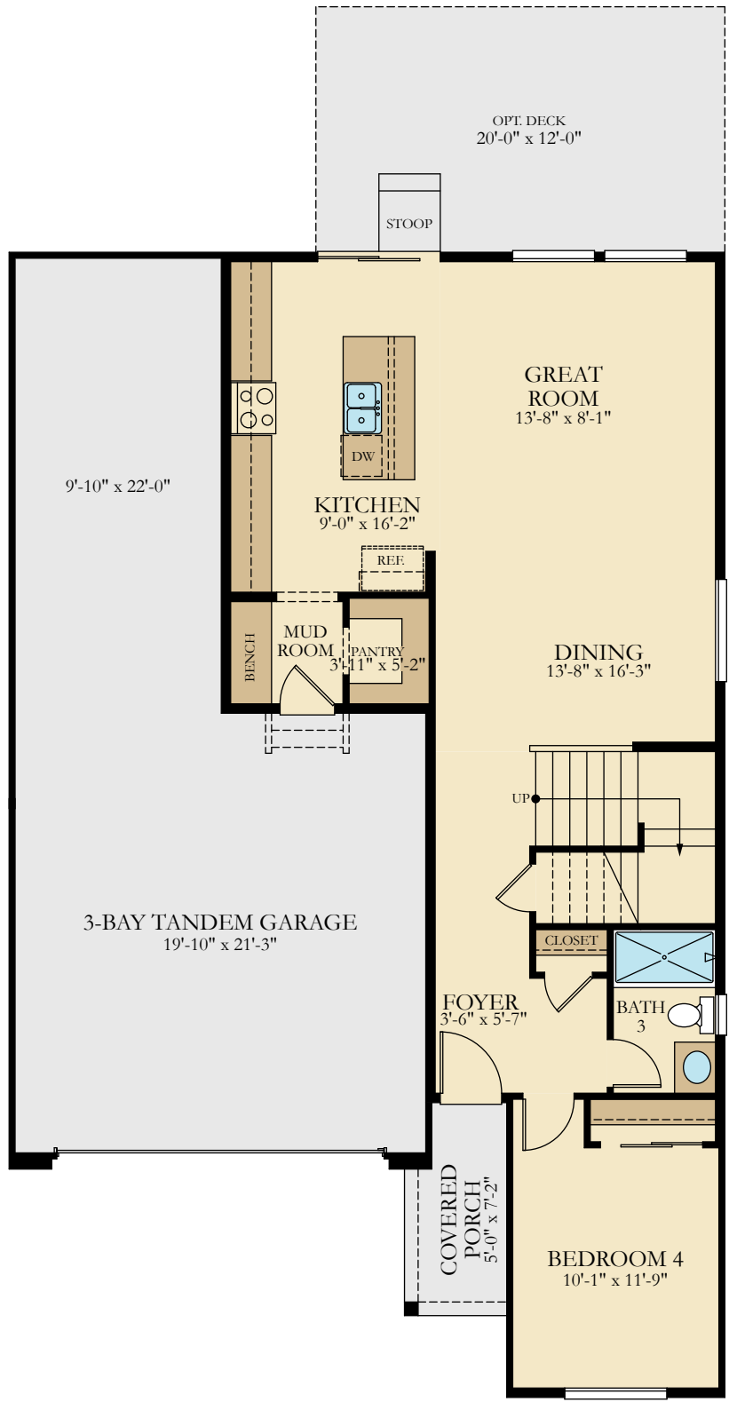
FIRST FLOOR
